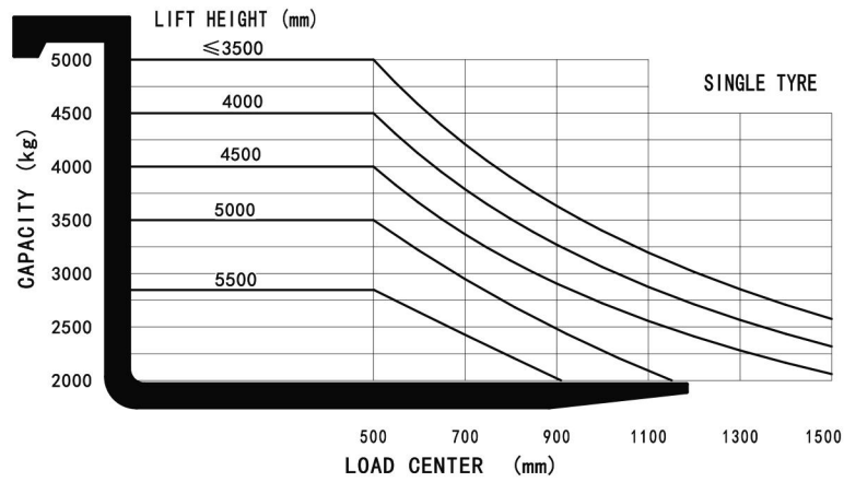
CAPACITY CHART
